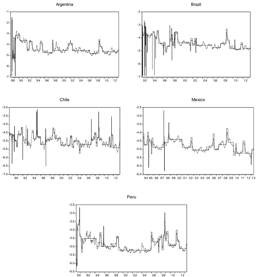
Figure 3. Level Shift Component \tau_t estimated by Bai and Perron (2003): solid line and Smoothed Level Shift Component: dotted line
