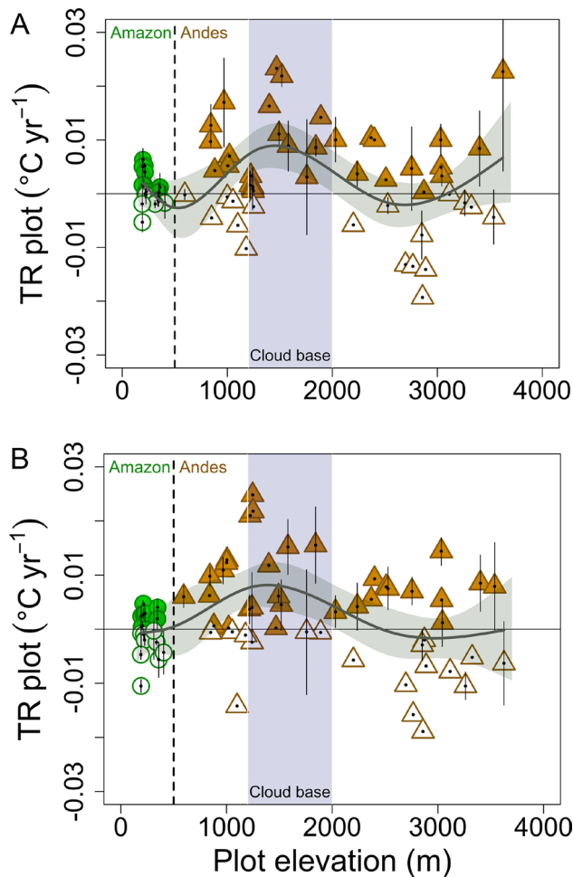
Fig. 3. The estimated plot-level TR for the 66 Amazonian and Andean forest plots with multiple censuses based on the (A) individual-weighted CTI and (B) basal area-weighted CTI. TR was calculated as the slope of the linear least-square regression between CTI and census year. Each circle (Amazon) or triangle (Andes) represents one forest plot; solid green and orange colors represent positive TR and empty green, and orange colors represent negative TR. Error bars represent the 95% CI based on the linear least-square regressions of the CTI versus the census year of each plot. Circles and triangles with no error bars represent plots with one census interval. The dashed vertical line indicates the approximate transition from Amazonian to Andean forests at 500 m. The solid green line is the GAM fit using the smoothing function with 95% CI. Vertical rectangles represent the approximate position of the cloud base along the gradient.
