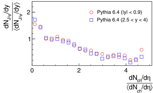
Fig. 4. Relative J/\psi yield dN_{J/\psi}/dy as a function of relative charged particle multiplicities around mid-rapidity dN_{ch}/d\eta as calculated with PYTHIA 6.4 in the Perugia 2011 tune [35,36]. Shown are results for directly produced J/\psi in hard scatterings via the NRQCD framework at forward rapidities ( 2.5 < y < 4 ) and at mid-rapidity ( |y| < 0.9 ).
