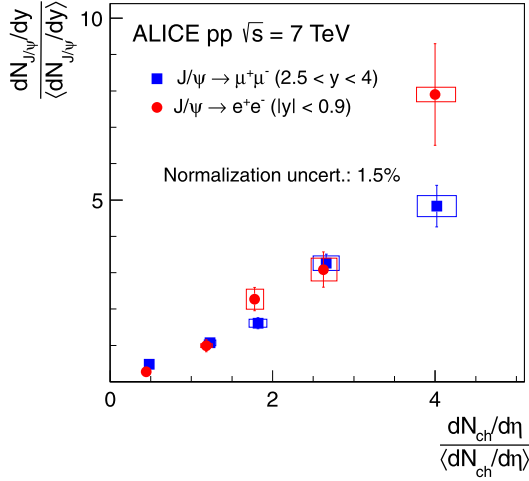
Fig. 3. J/\psi yield dN_{J/\psi}/dy as a function of the charged particle multiplicities at mid-rapidity dN_{ch}/d\eta . Both values are normalized by the corresponding value for minimum bias pp collisions ( (dN_{J/\psi}/dy) , (dN_{ch}/d\eta) ). Shown are measurements at forward rapidities ( J/\psi \rightarrow \mu^+\mu^- , 2.5 < y < 4 ) and at mid-rapidity ( J/\psi \rightarrow e^+e^- , |y| < 0.9 ). The error bars represent the statistical uncertainty on the J/\psi yields, while the quadratic sum of the point-by-point systematic uncertainties on the J/\psi yield as well as on dN_{ch}/d\eta is depicted as boxes.
