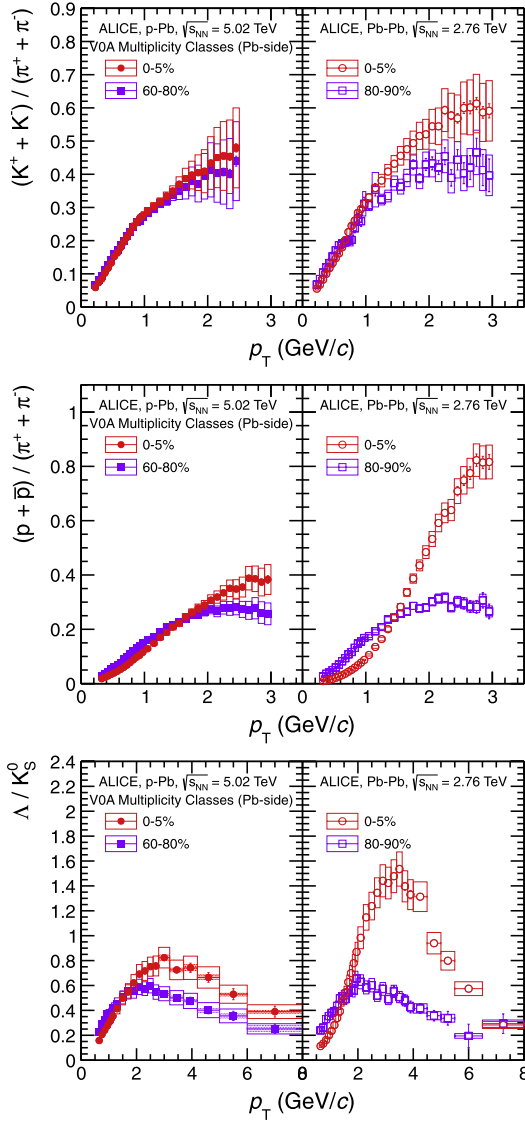
Fig. 2. (Color online.) Ratios K/\pi = (K^+ + K^-)/(\pi^+ + \pi^-) and \Lambda/K_S^0 as a function of p_T in two multiplicity bins measured in the rapidity interval 0 < y_{\text{CMS}} < 0.5 (left panels). The ratios are compared to results in Pb-Pb collisions measured at mid-rapidity, shown in the right panels. The empty boxes show the total systematic uncertainty; the shaded boxes indicate the contribution uncorrelated across multiplicity bins (not estimated in Pb-Pb).
