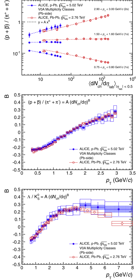
Fig. 3. (Color online.) p/\pi ratio as a function of the charged-particle density dN_{\text{ch}}/d\eta in three p_T intervals in p-Pb (measured in the rapidity interval 0 < y_{\text{CMS}} < 0.5 ) and Pb-Pb collisions (measured at mid-rapidity). The dashed lines show the corresponding power-law fit (top). Exponent of the p/\pi (middle) and \Lambda/K_S^0 (bottom) power-law fit as a function of p_T in p-Pb and Pb-Pb collisions. The empty boxes show the total systematic uncertainty; the shaded boxes indicate the contribution uncorrelated across multiplicity bins (not estimated in Pb-Pb).
