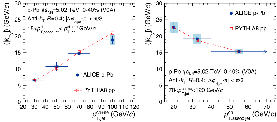
Fig. 3. Mean of the |k_{Ty}| distributions as a function of the full jet transverse momentum p_{T,jet}^{ch+ne} (left) and the associated charged jet transverse momentum p_{T,assoc jet}^{ch} (right) compared to PYTHIA8.
