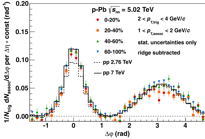
Fig. 5. Associated yield per trigger particle as a function of \Delta\phi averaged over |\Delta\eta| < 1.8 for pairs of charged particles with 2 < p_{T,\text{trig}} < 4 GeV/c and 1 < p_{T,\text{assoc}} < 2 GeV/c in p-Pb collisions at \sqrt{s_{NN}} = 5.02 TeV for different event classes, compared to pp collisions at \sqrt{s} = 2.76 and 7 TeV. For the event classes 0–20%, 20–40% and 40–60% the long-range contribution on the near-side 1.2 < |\Delta\eta| < 1.8 and |\Delta\phi| < \pi/2 has been subtracted from both the near side and the away side as described in the text. Subsequently, the yield between the peaks (determined at \Delta\phi \approx 1.3 ) has been subtracted in each case. Only statistical uncertainties are shown; systematic uncertainties are less than 0.01 (absolute) per bin.
