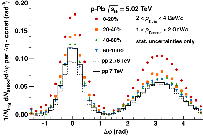
Fig. 2. Associated yield per trigger particle as a function of \Delta\phi averaged over |\Delta\eta| < 1.8 for pairs of charged particles with 2 < p_{T,\text{trig}} < 4 GeV/c and 1 < p_{T,\text{assoc}} < 2 GeV/c in p-Pb collisions at \sqrt{s_{\text{NN}}} = 5.02 TeV for different event classes, and in pp collisions at 2.76 and 7 TeV. The yield between the peaks (determined at \Delta\phi \approx 1.3 ) has been subtracted in each case. Only statistical uncertainties are shown; systematic uncertainties are less than 0.01 (absolute) per bin.
