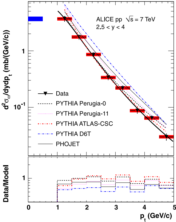
Fig. 6. (Colour online.) Top: Inclusive differential \omega production cross section d^2\sigma_\omega/dydp_t for 2.5 < y < 4 . The error bars represent the quadratic sum of the statistical and systematic uncertainties, the red boxes the point-to-point uncorrelated systematic uncertainty, the blue box on the left the error on normalization. Data are fitted with Eq. (1) (solid line) and compared with the Perugia-0, Perugia-11, ATLAS-CSC and D6T PYTHIA tunes and PHOJET. Bottom: Ratio between data and models.
