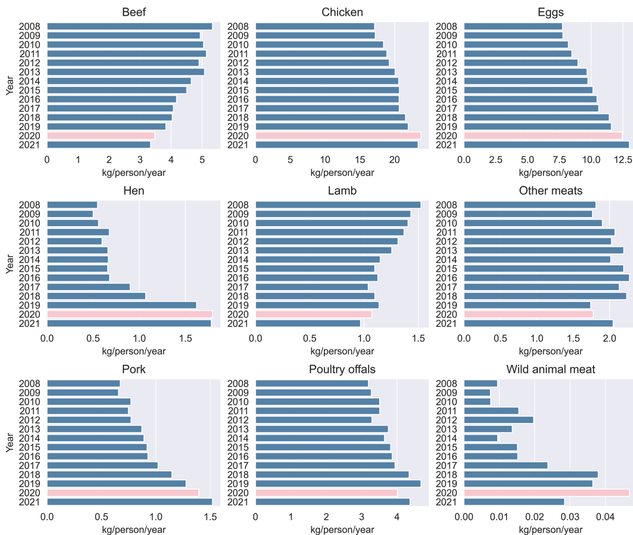
FIGURE 3 Trends in per capita consumption of the main animal-based protein sources in Peru in the period 2008–2021. The pink bar indicates the year of the pandemic (2020). Underlying data for this figure are available in Table SM2 of Supporting Information S2.
