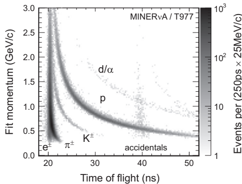
Fig. 2. The measured momentum and time-of-flight used to separate different particle species and backgrounds. The origin of the backgrounds from the accelerator timing structure are described in the text.
